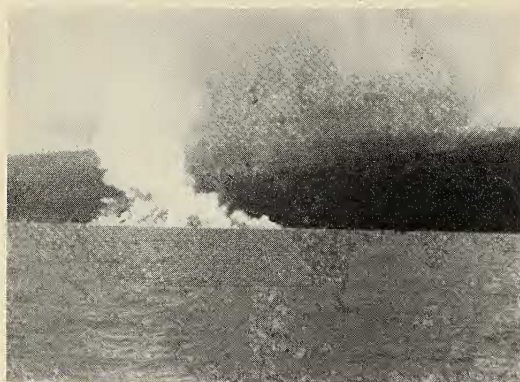
FIG. 2. Third lava flow reaching sea level on June 3.
